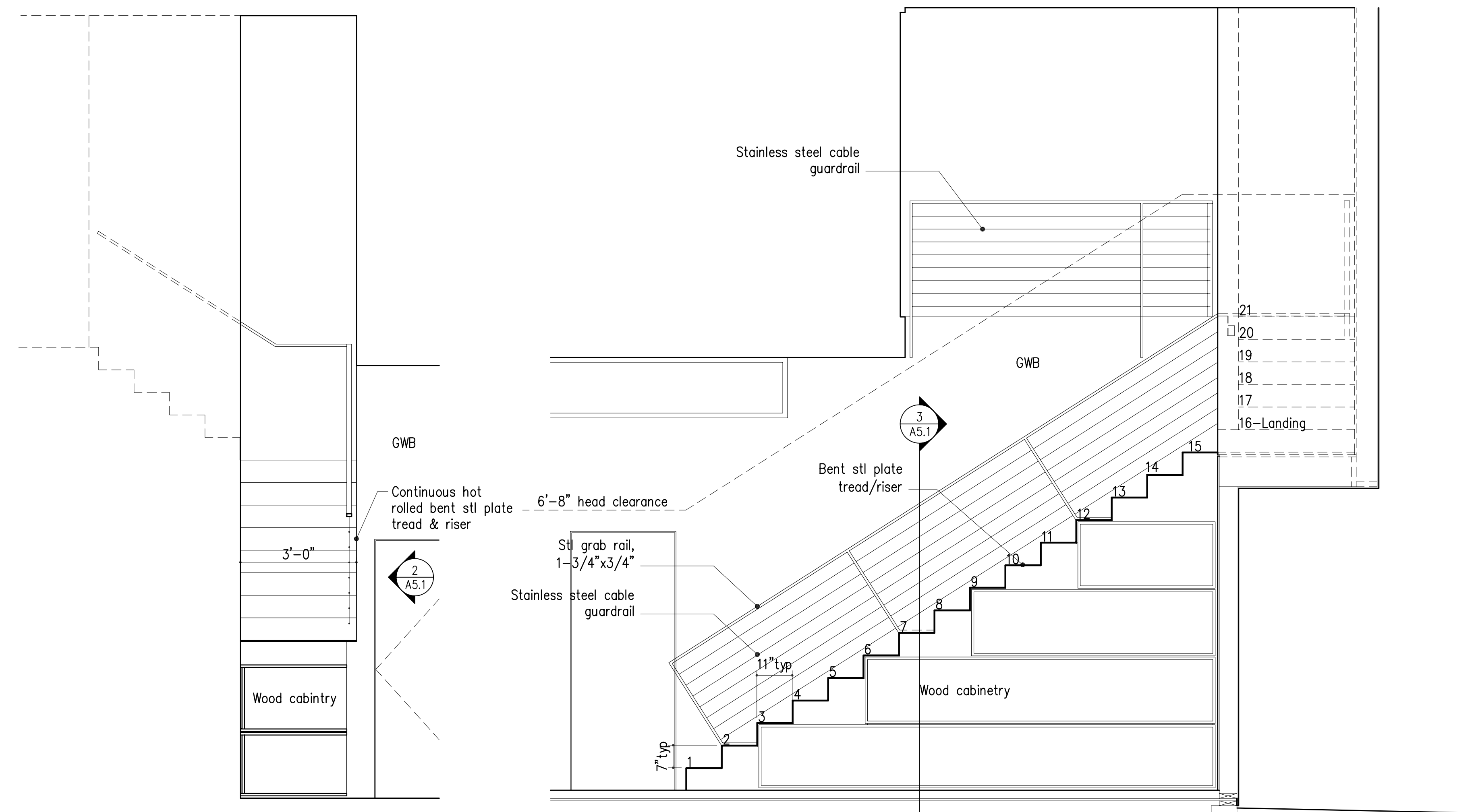
3 DETAIL STAIR SECTION A5.1 scale: 1/2" = 1'-0"
