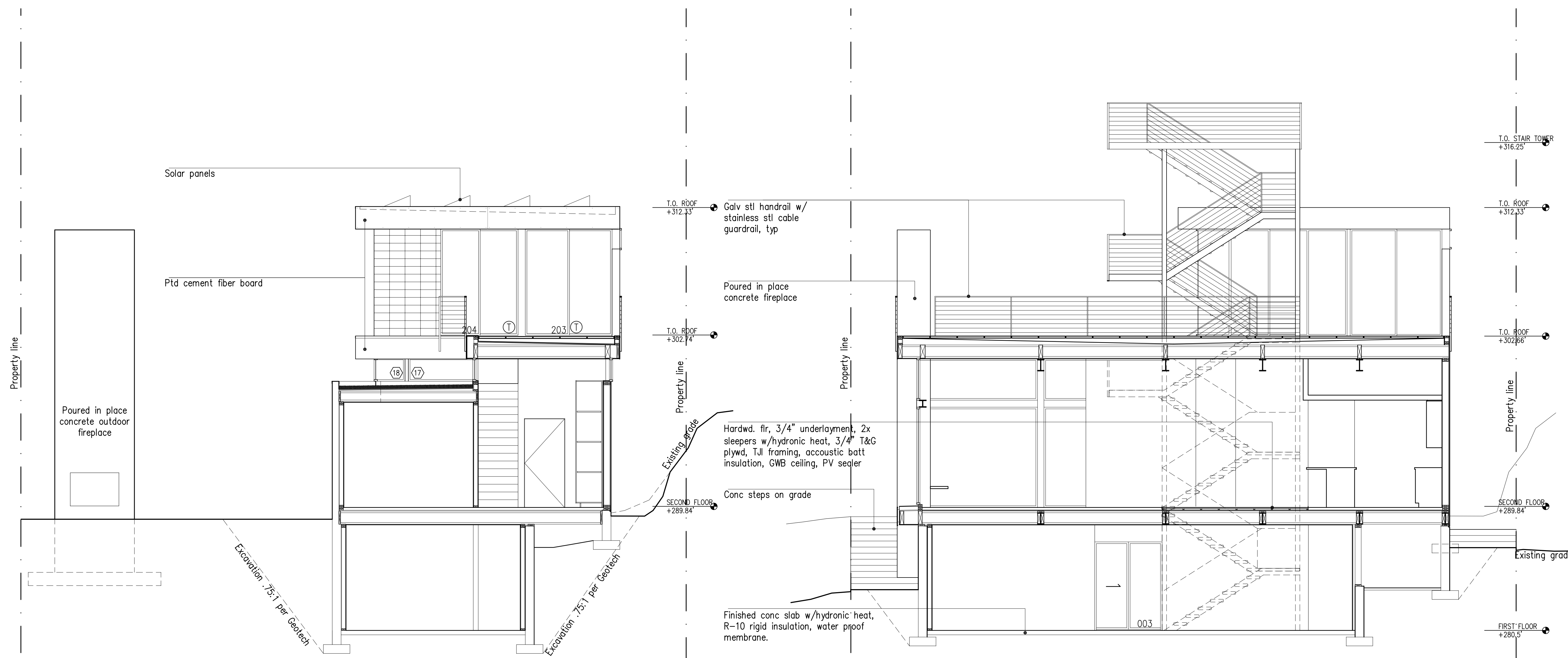
2 NORTH SOUTH SECTION A3.1 scale: 1/4" = 1'-0"
