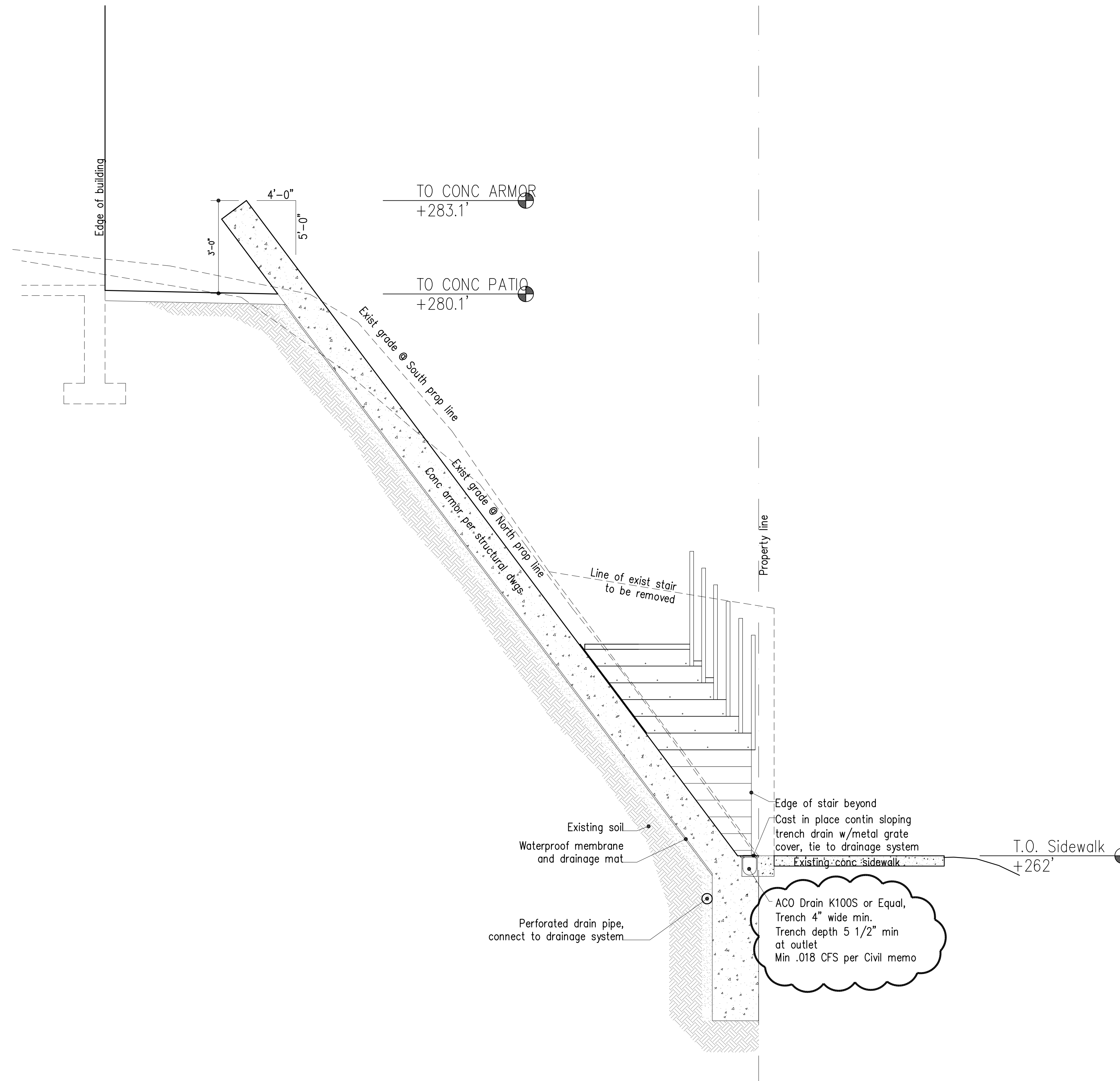
1 SECTION @ ARMORED WALL A0.3 scale: 1/2"=1'-0"
